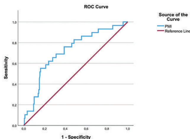
Figure 1. ROC curve.
